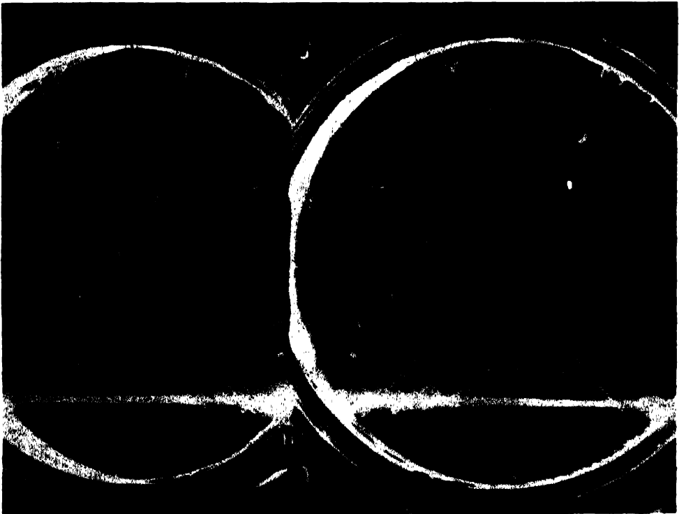
FIG. 1. CLOUD CHAMBER TRACKS
